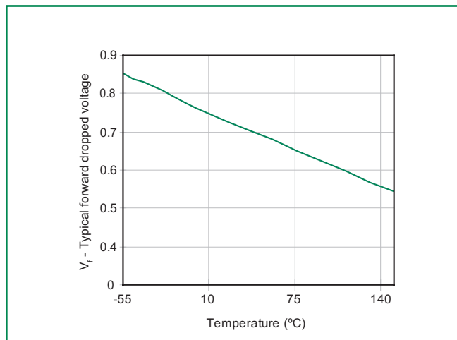
Figure 6 - Forward Voltage
