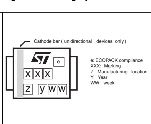
Figure 14. Marking layout (1)
