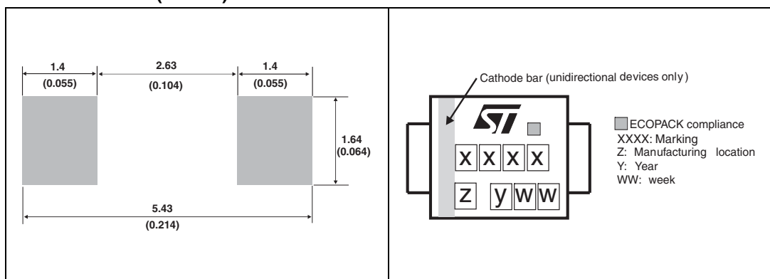
Figure 17. SMA footprint dimensions in mm (inches) Figure 18. Marking layout (1)
