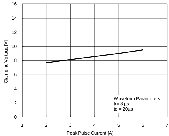
I/O Clamping Voltage vs. Peak Pulse Current
