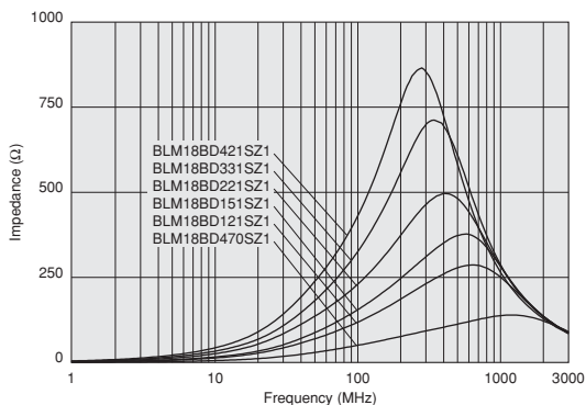
BLM18BD_SZ Series (47Ω~420Ω)
