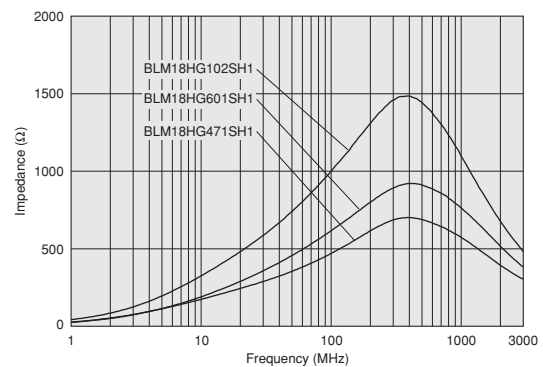
BLM18HG_SH Series (For General Signal Lines)
