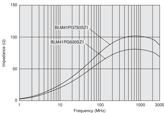
BLM41PG_SZ Series (60Ω~75Ω)
