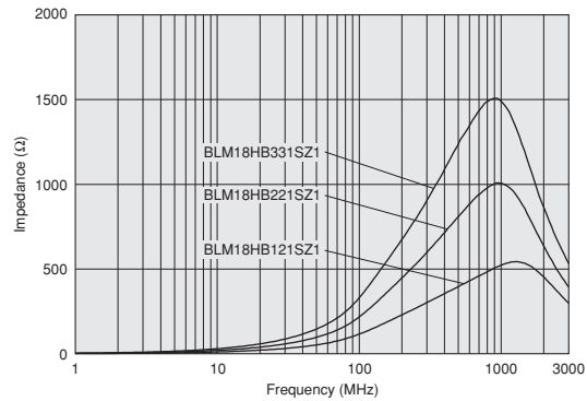
BLM18HB_SZ Series (For High Speed Signal Lines)
