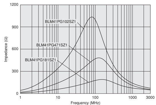
BLM41PG_SZ Series (180Ω~1000Ω)
