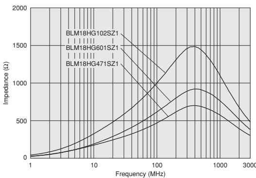
BLM18HG_SZ Series (For General Signal Lines)
