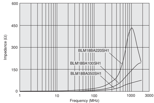
BLM18BA_SH Series (5Ω~22Ω)
