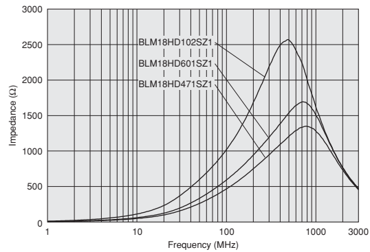
BLM18HD_SZ Series (For High Speed Signal Lines)
