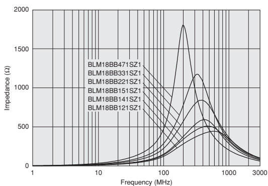
BLM18BB_SZ Series (120Ω~470Ω)
