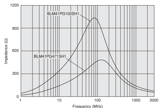
BLM41PG_SH Series (470Ω~1000Ω)
