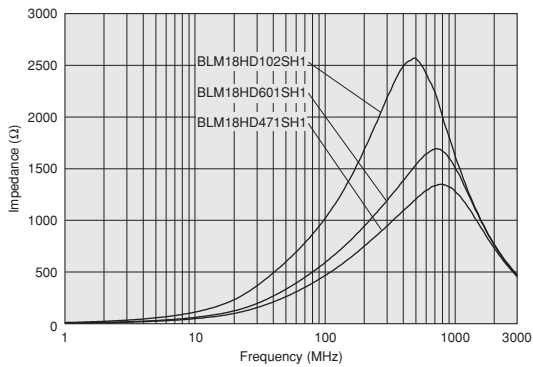
BLM18HD_SH Series (For High Speed Signal Lines)
