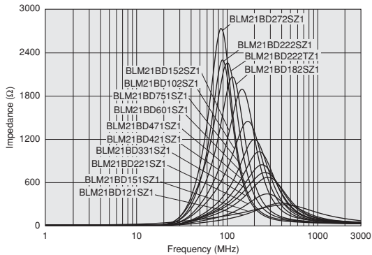
BLM21BD_SZ, TZ Series
