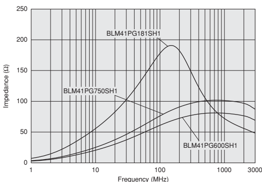
BLM41PG_SH Series (60Ω~180Ω)
