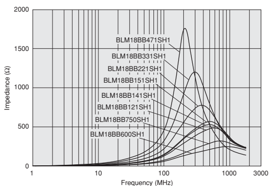
BLM18BB_SH Series (60Ω~470Ω)
