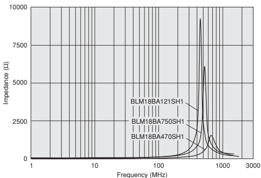
BLM18BA_SH Series (47Ω~120Ω)
